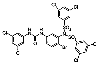
Compound # 29
